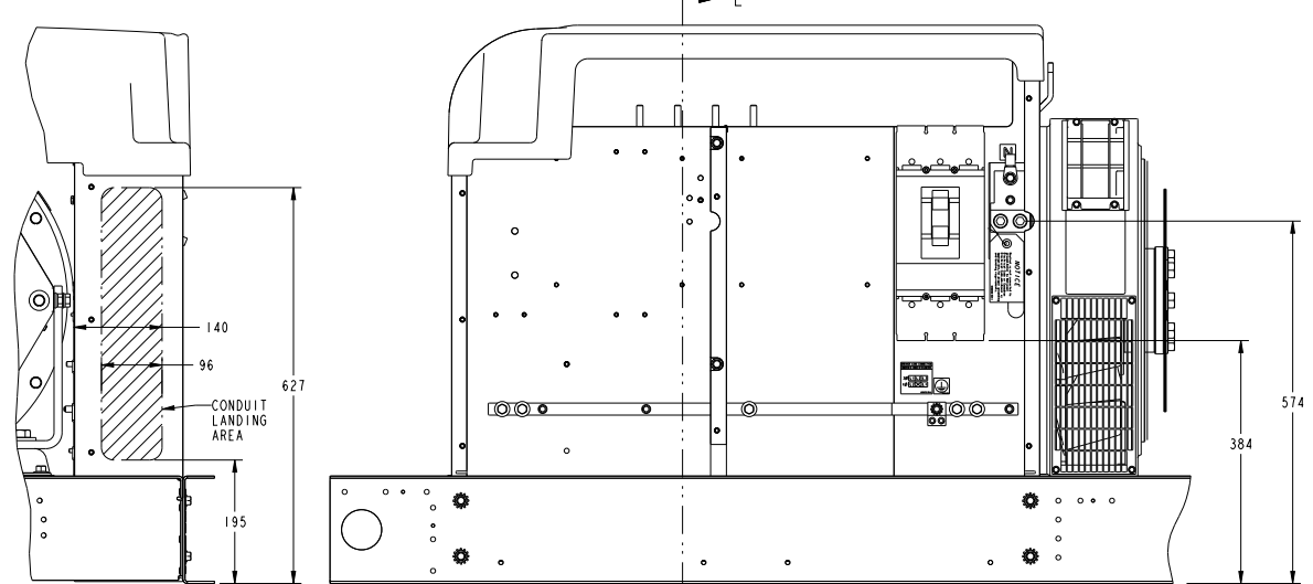
"L" FRAME SHOWN (400 - 600 amp)
